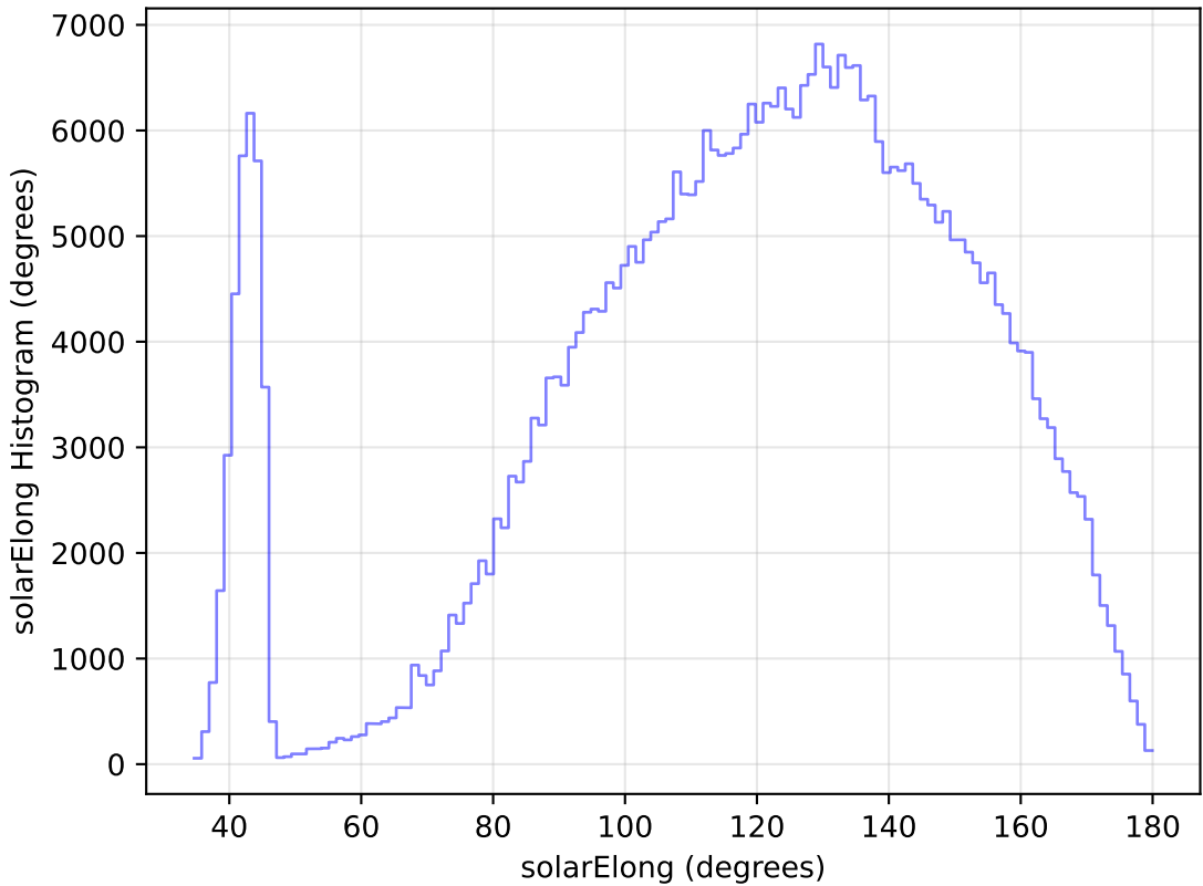
extra_ss_neo3_v3.4_10yrs WFD z band: solarElong Histogram
