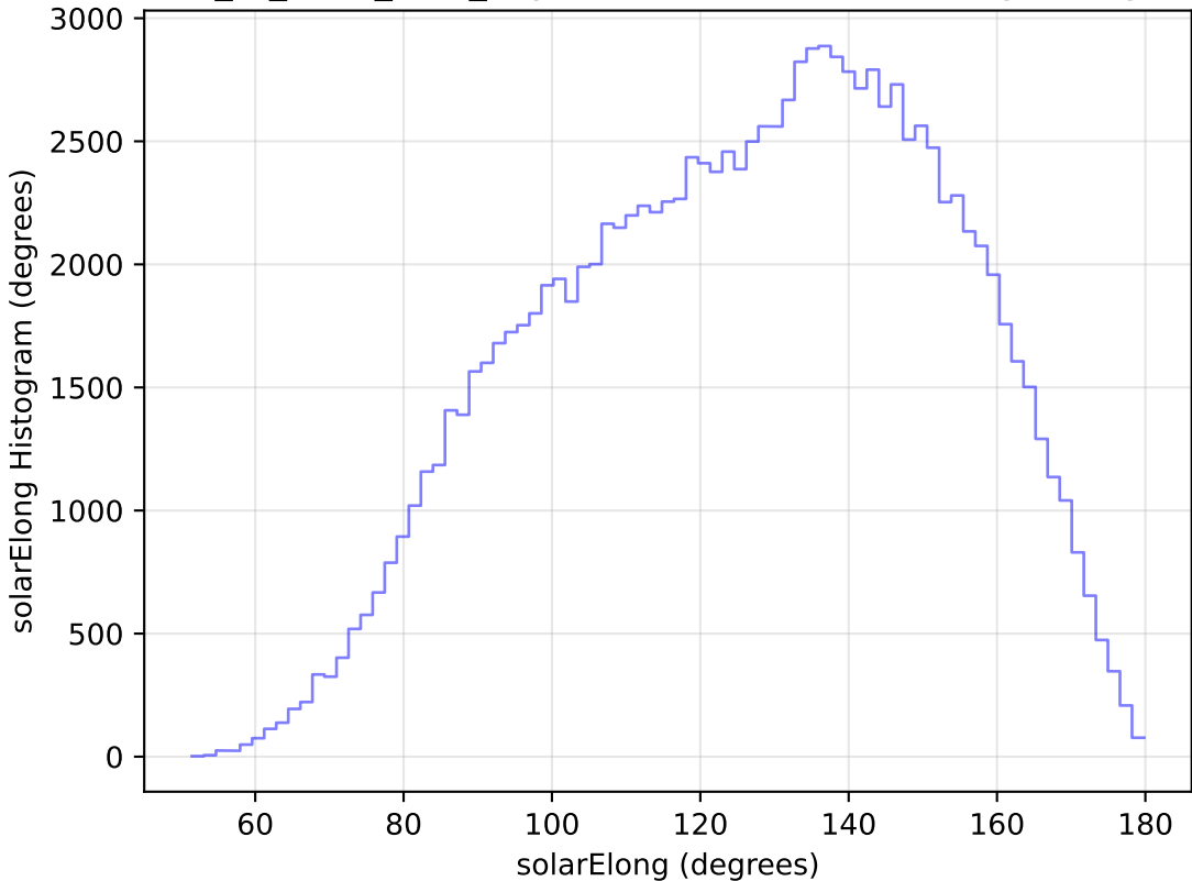
extra_ss_neo3_v3.4_10yrs WFD u band: solarElong Histogram
