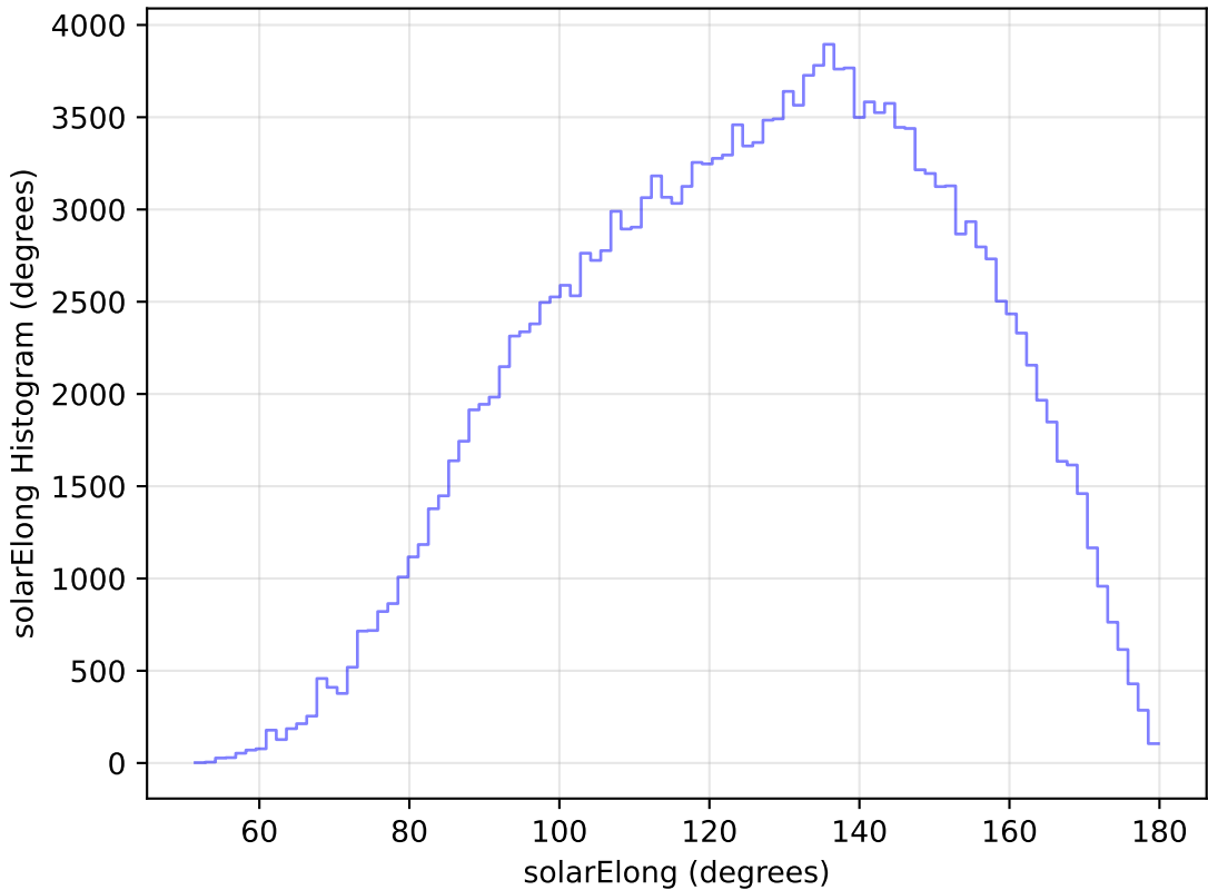
extra_ss_neo3_v3.4_10yrs WFD g band: solarElong Histogram
