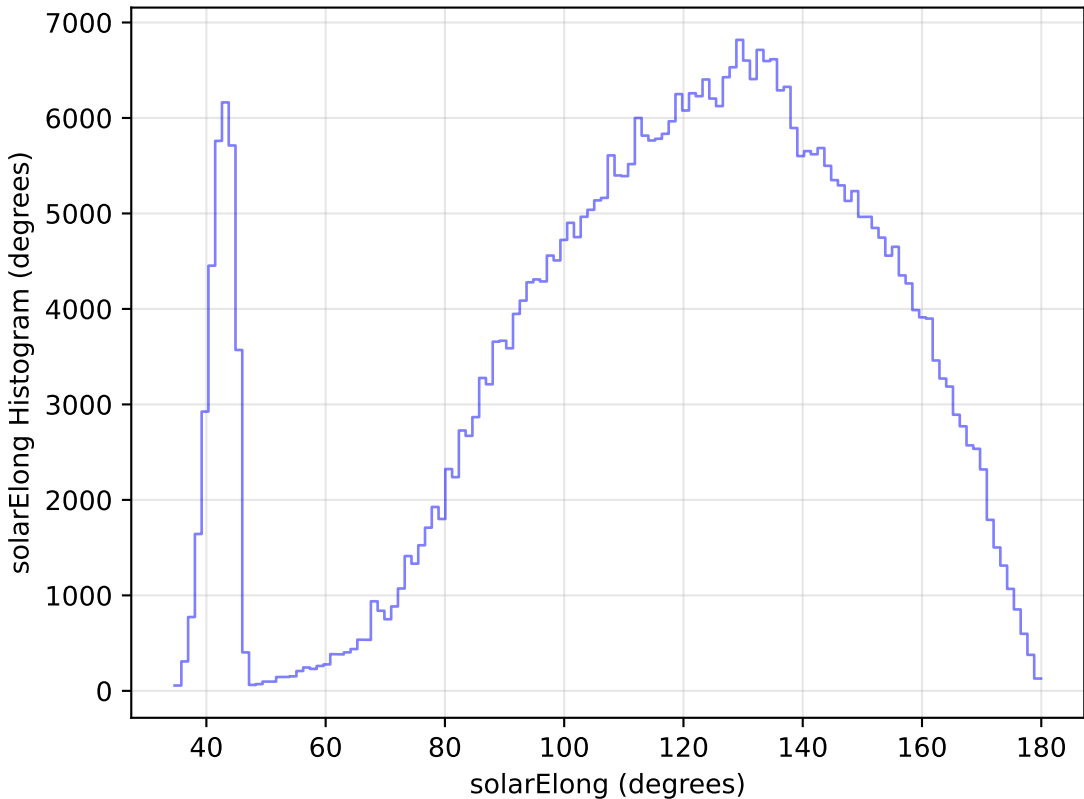
extra_ss_neo3_v3.4_10yrs All sky z band: solarElong Histogram
