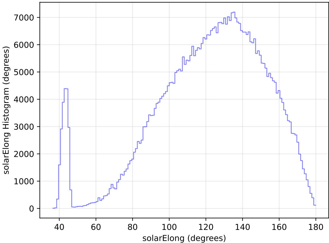
extra_ss_neo3_v3.4_10yrs All sky r band: solarElong Histogram
