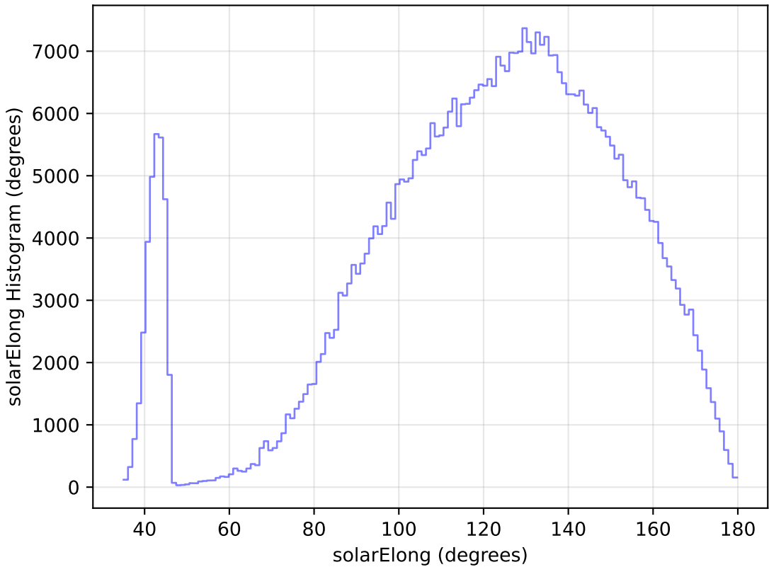
extra_ss_neo3_v3.4_10yrs All sky i band: solarElong Histogram
