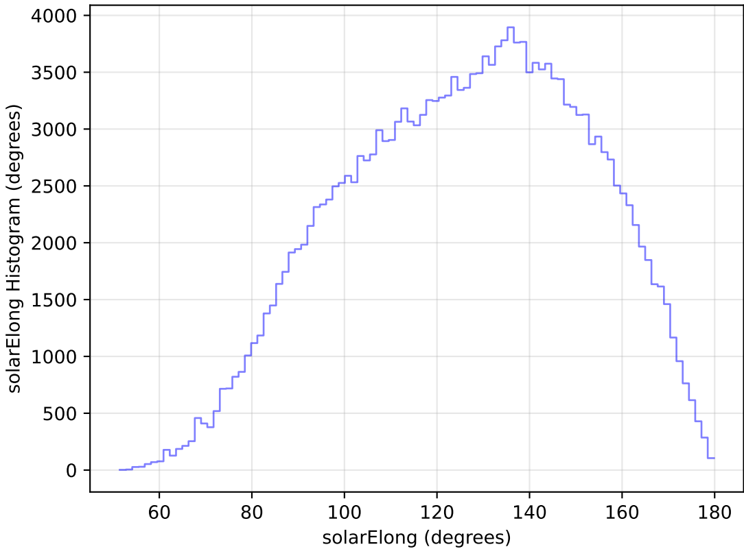
extra_ss_neo3_v3.4_10yrs All sky g band: solarElong Histogram
