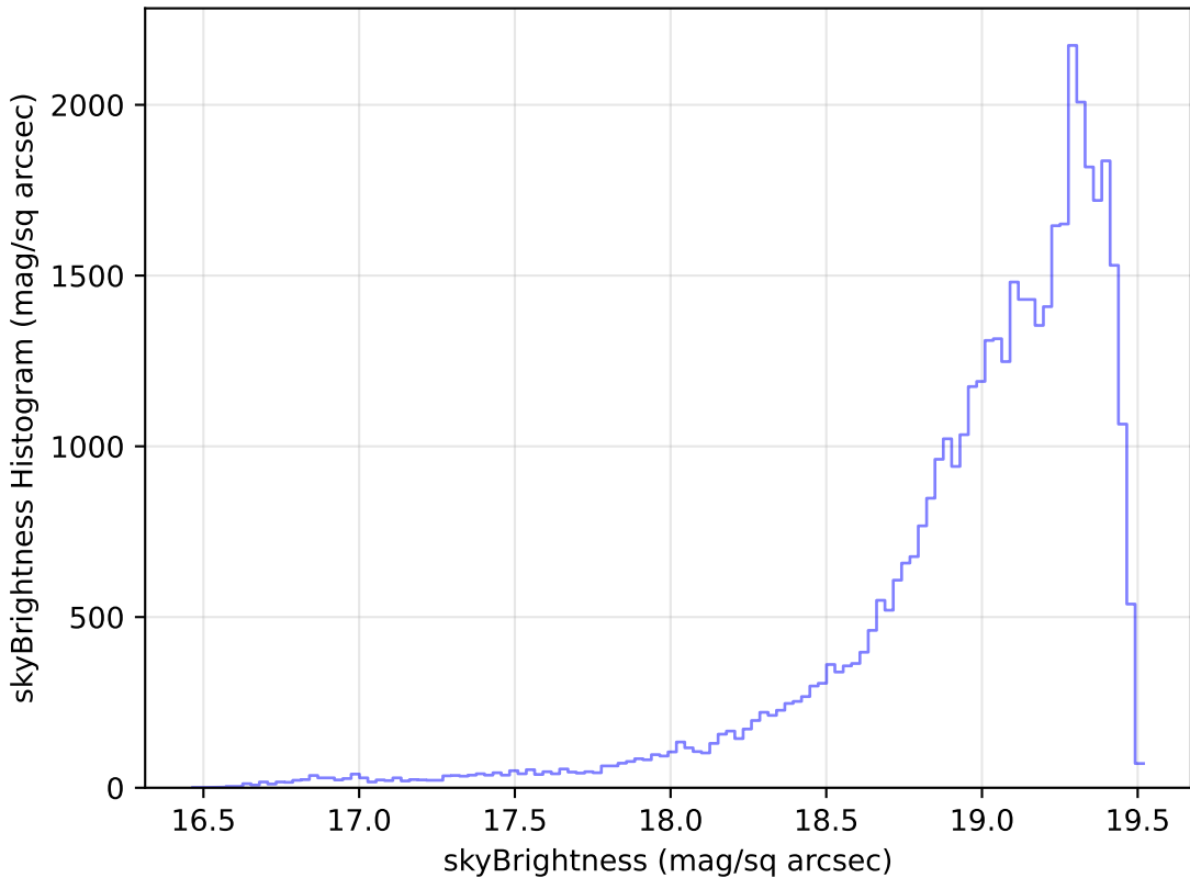
extra_ss_neo3_v3.4_10yrs Yr 1 z band: skyBrightness Histogram
