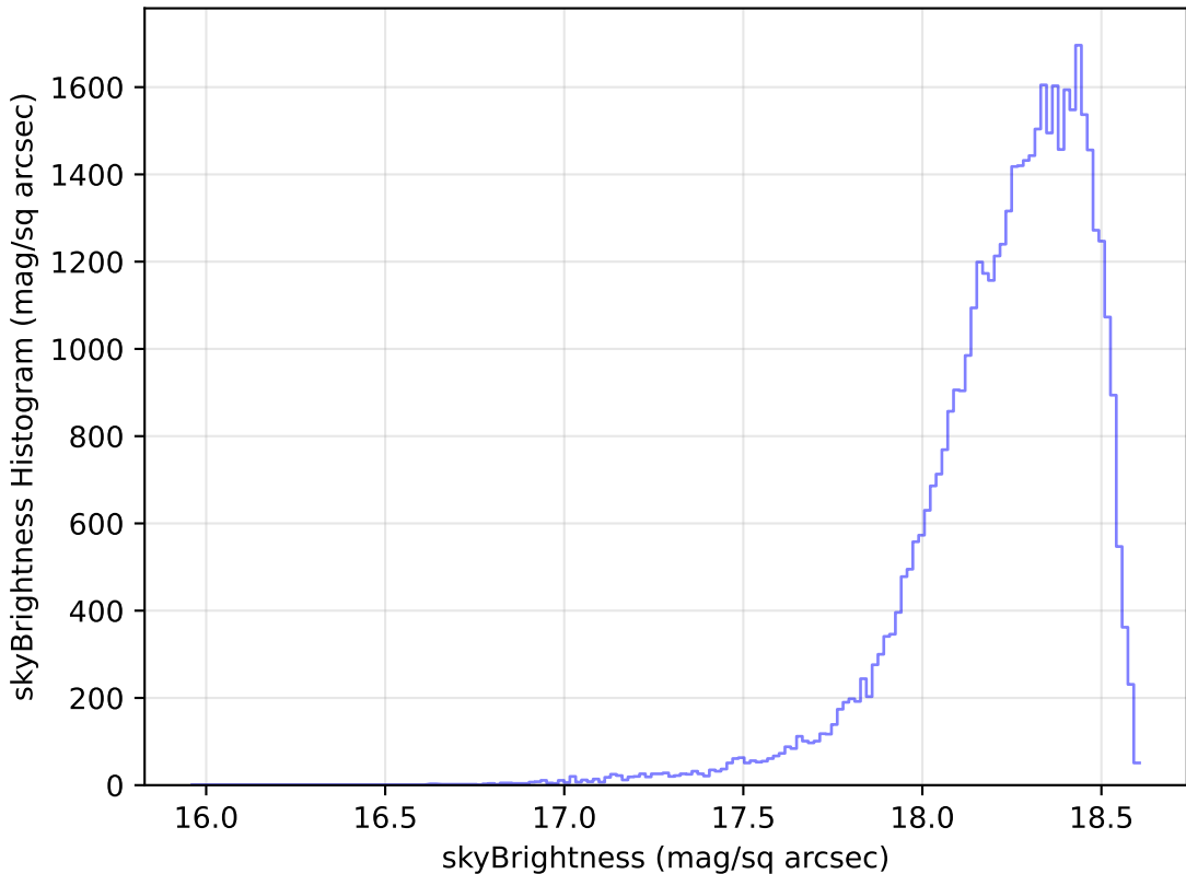
extra_ss_neo3_v3.4_10yrs Yr 1 y band: skyBrightness Histogram
