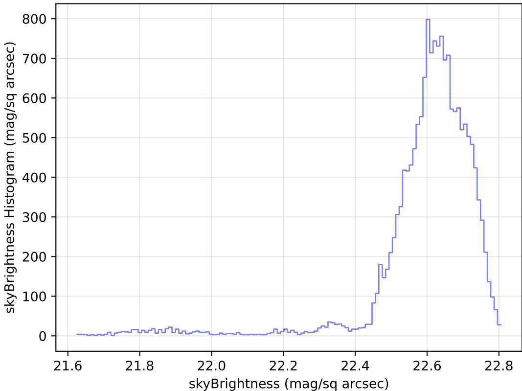
extra_ss_neo3_v3.4_10yrs Yr 1 u band: skyBrightness Histogram
