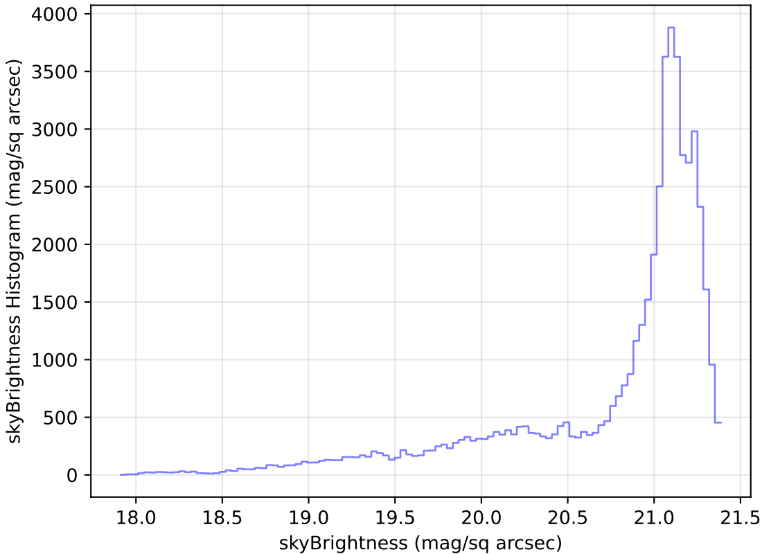
extra_ss_neo3_v3.4_10yrs Yr 1 r band: skyBrightness Histogram
