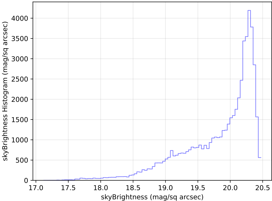
extra_ss_neo3_v3.4_10yrs Yr 1 i band: skyBrightness Histogram
