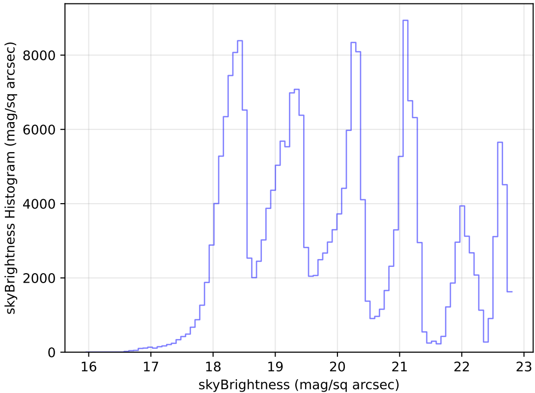
extra_ss_neo3_v3.4_10yrs Yr 1 all bands: skyBrightness Histogram
