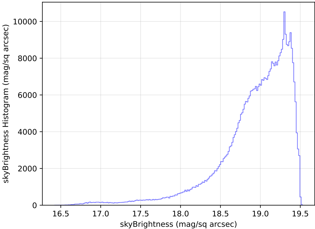
extra_ss_neo3_v3.4_10yrs WFD z band: skyBrightness Histogram
