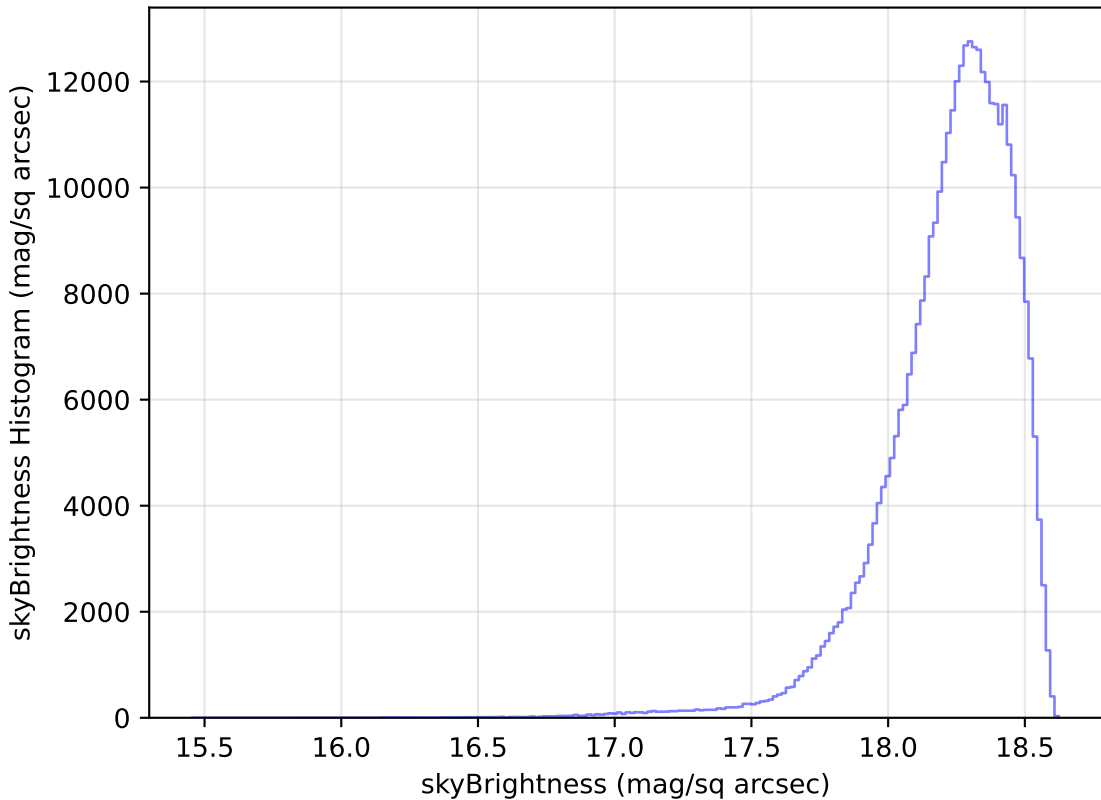
extra_ss_neo3_v3.4_10yrs WFD y band: skyBrightness Histogram
