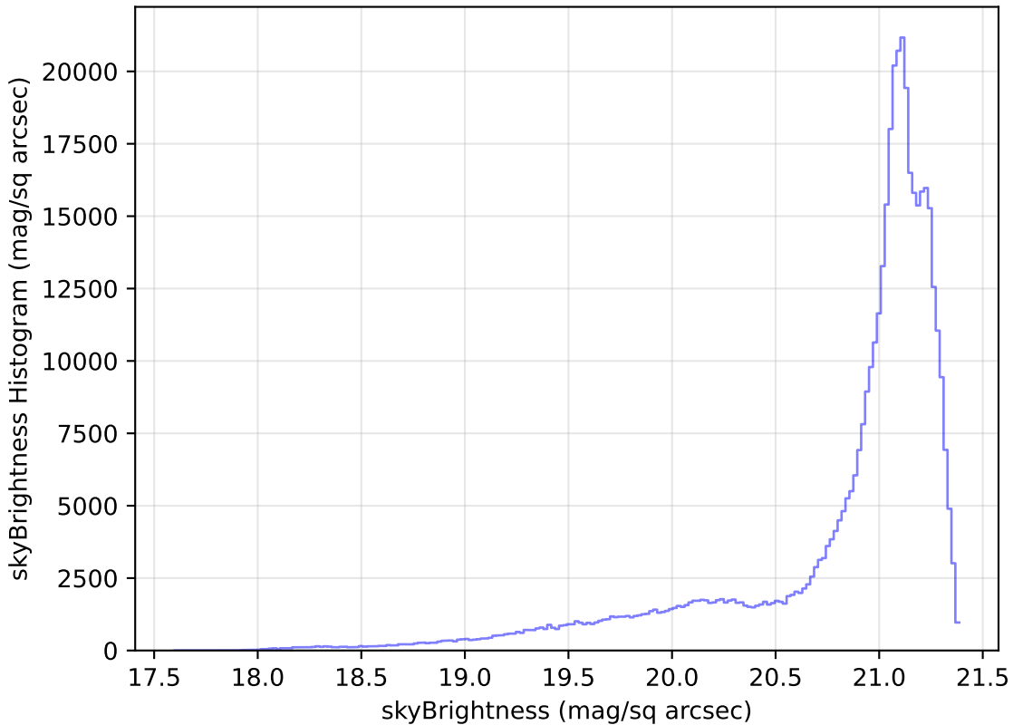
extra_ss_neo3_v3.4_10yrs WFD r band: skyBrightness Histogram
