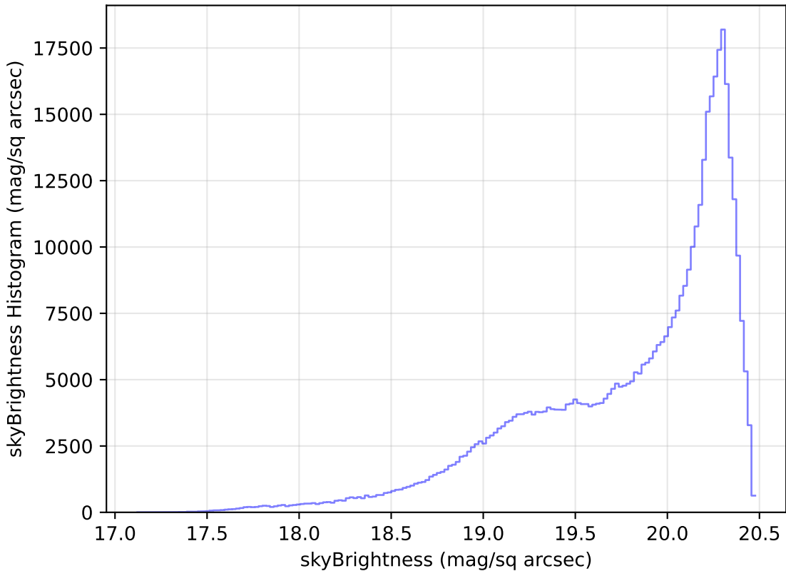
extra_ss_neo3_v3.4_10yrs WFD i band: skyBrightness Histogram
