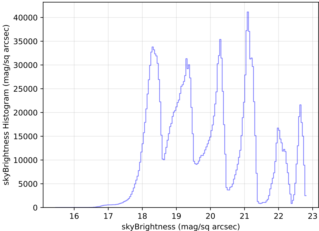
extra_ss_neo3_v3.4_10yrs WFD all bands: skyBrightness Histogram
