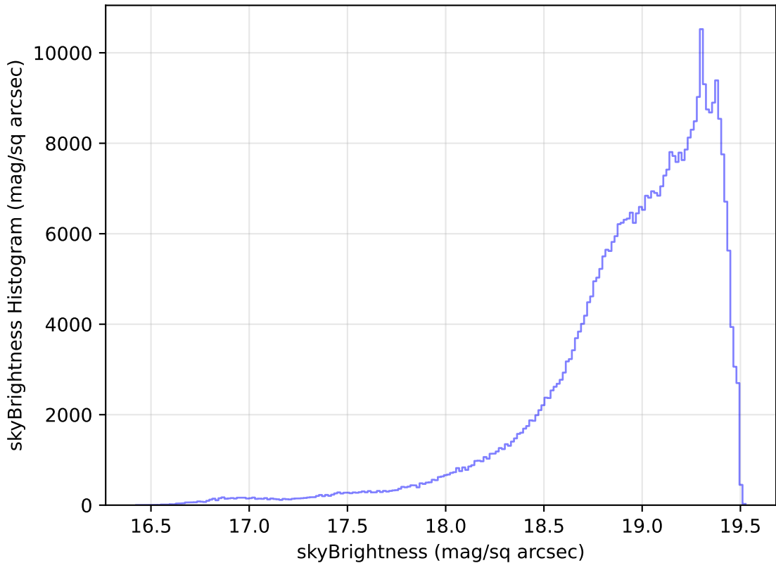
extra_ss_neo3_v3.4_10yrs All sky z band: skyBrightness Histogram
