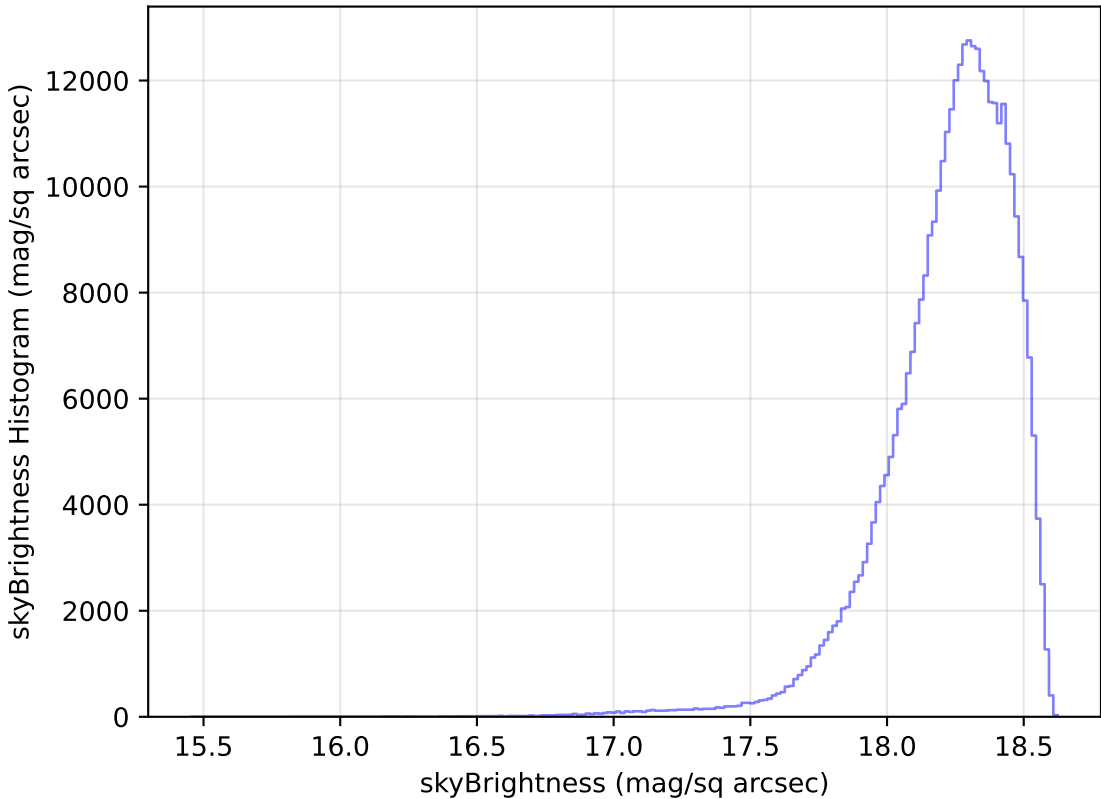
extra_ss_neo3_v3.4_10yrs All sky y band: skyBrightness Histogram
