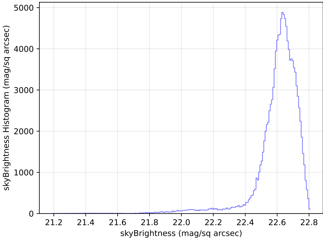
extra_ss_neo3_v3.4_10yrs All sky u band: skyBrightness Histogram
