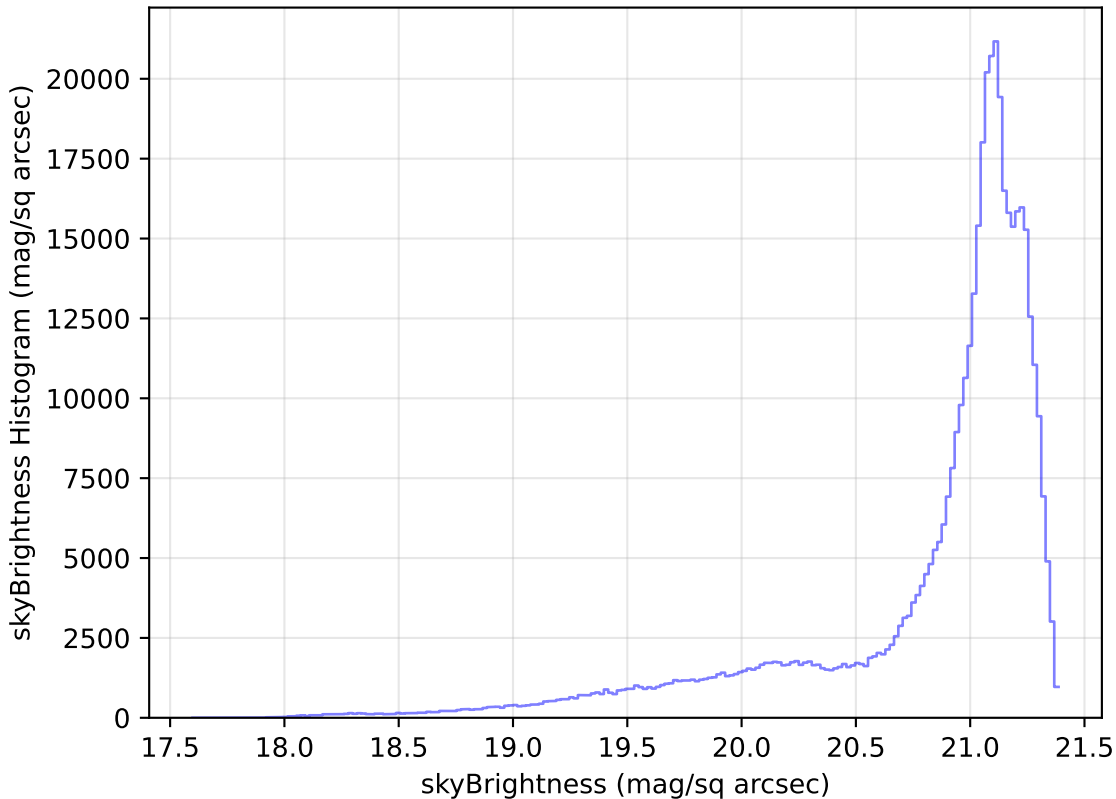
extra_ss_neo3_v3.4_10yrs All sky r band: skyBrightness Histogram
