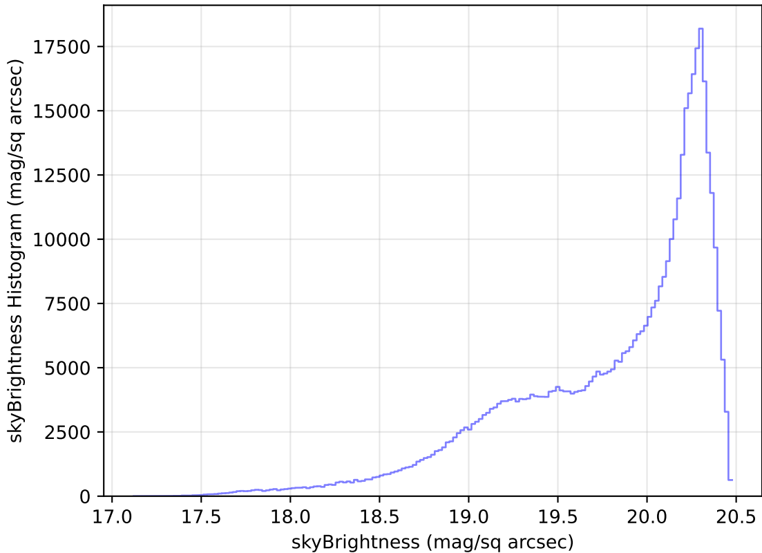
extra_ss_neo3_v3.4_10yrs All sky i band: skyBrightness Histogram
