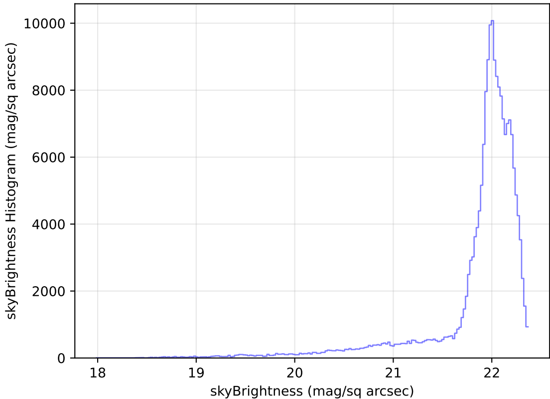
extra_ss_neo3_v3.4_10yrs All sky g band: skyBrightness Histogram
