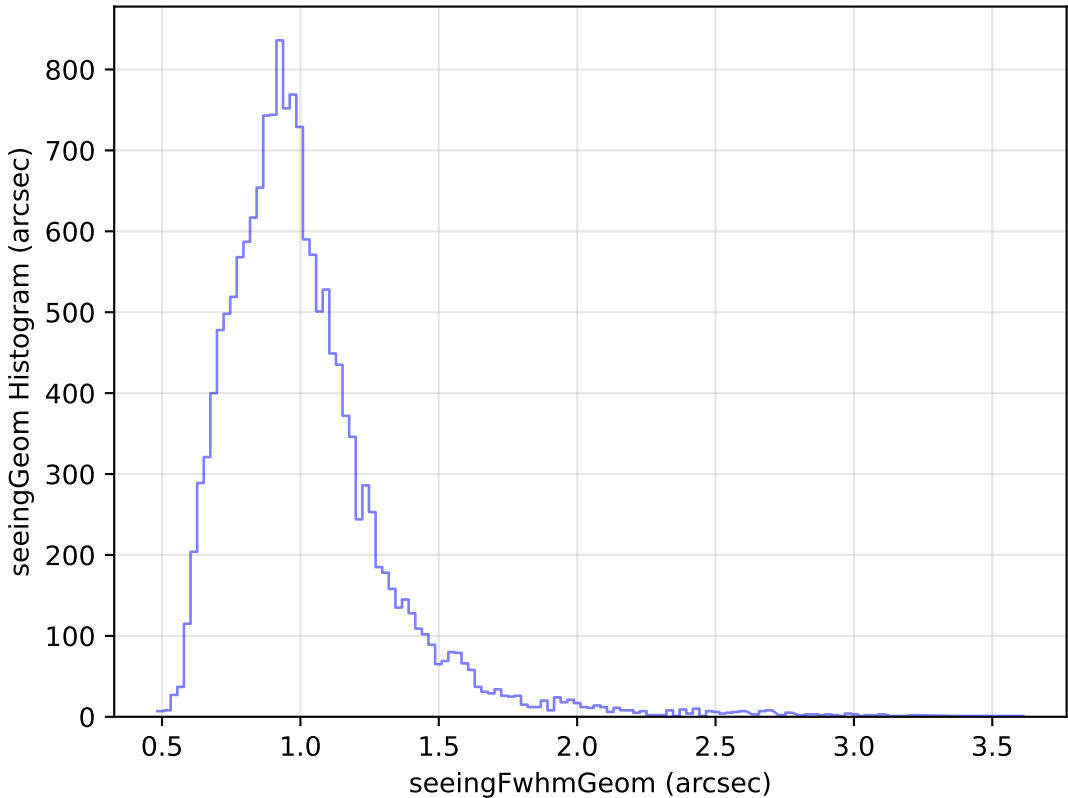
extra_ss_neo3_v3.4_10yrs Yr 1 u band: seeingGeom Histogram
