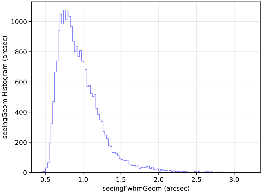
extra_ss_neo3_v3.4_10yrs Yr 1 g band: seeingGeom Histogram
