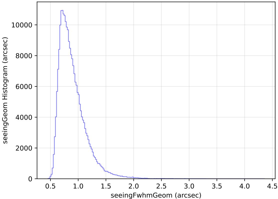
extra_ss_neo3_v3.4_10yrs Yr 1 all bands: seeingGeom Histogram
