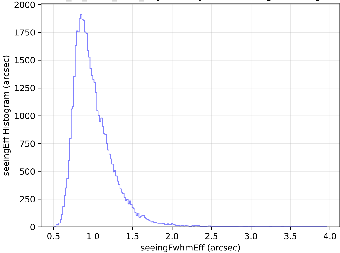
extra_ss_neo3_v3.4_10yrs Yr 1 y band: seeingEff Histogram
