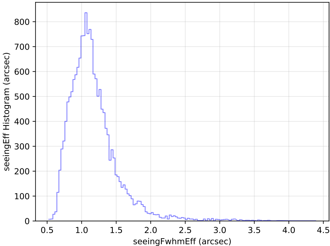
extra_ss_neo3_v3.4_10yrs Yr 1 u band: seeingEff Histogram
