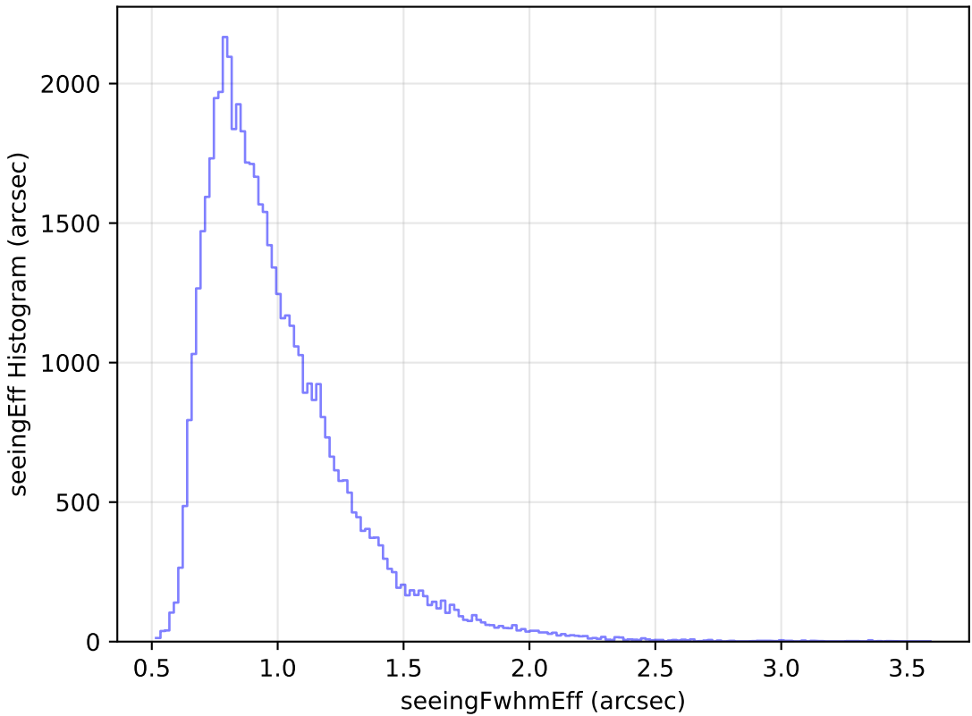
extra_ss_neo3_v3.4_10yrs Yr 1 i band: seeingEff Histogram
