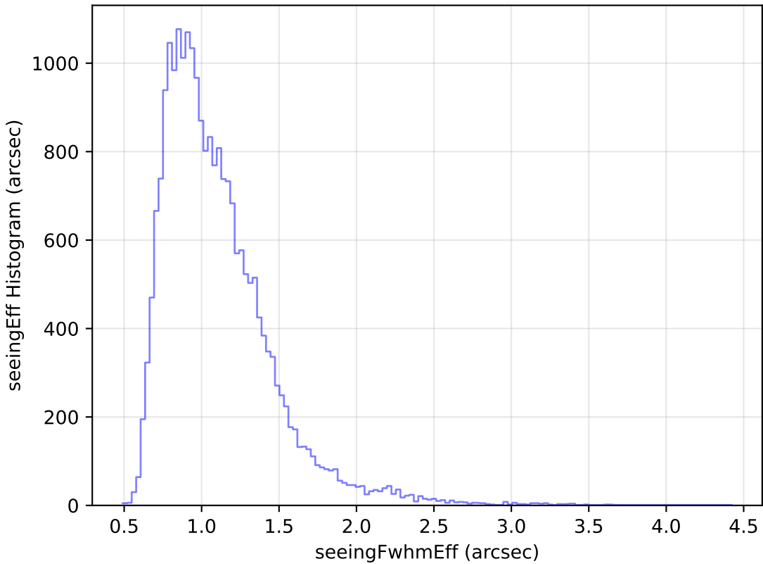
extra_ss_neo3_v3.4_10yrs Yr 1 g band: seeingEff Histogram
