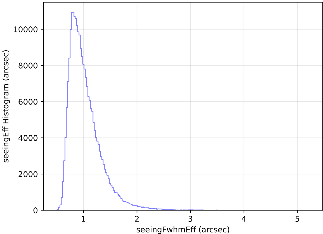
extra_ss_neo3_v3.4_10yrs Yr 1 all bands: seeingEff Histogram
