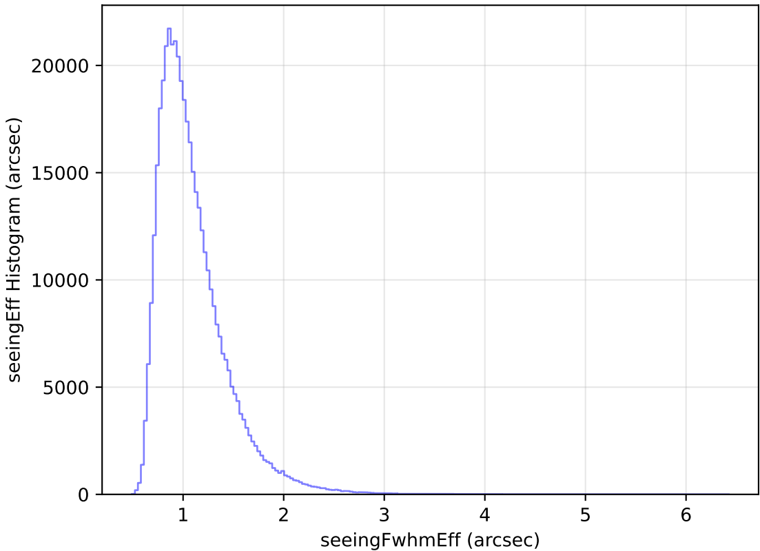
extra_ss_neo3_v3.4_10yrs WFD z band: seeingEff Histogram
