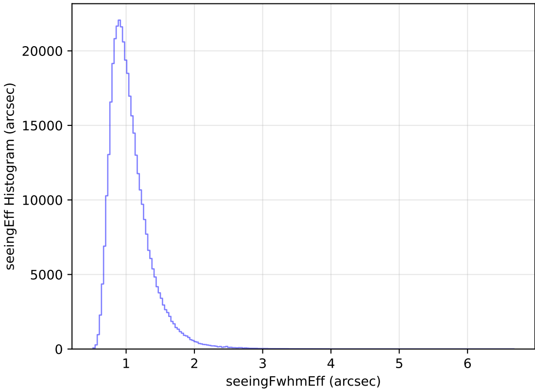
extra_ss_neo3_v3.4_10yrs WFD y band: seeingEff Histogram
