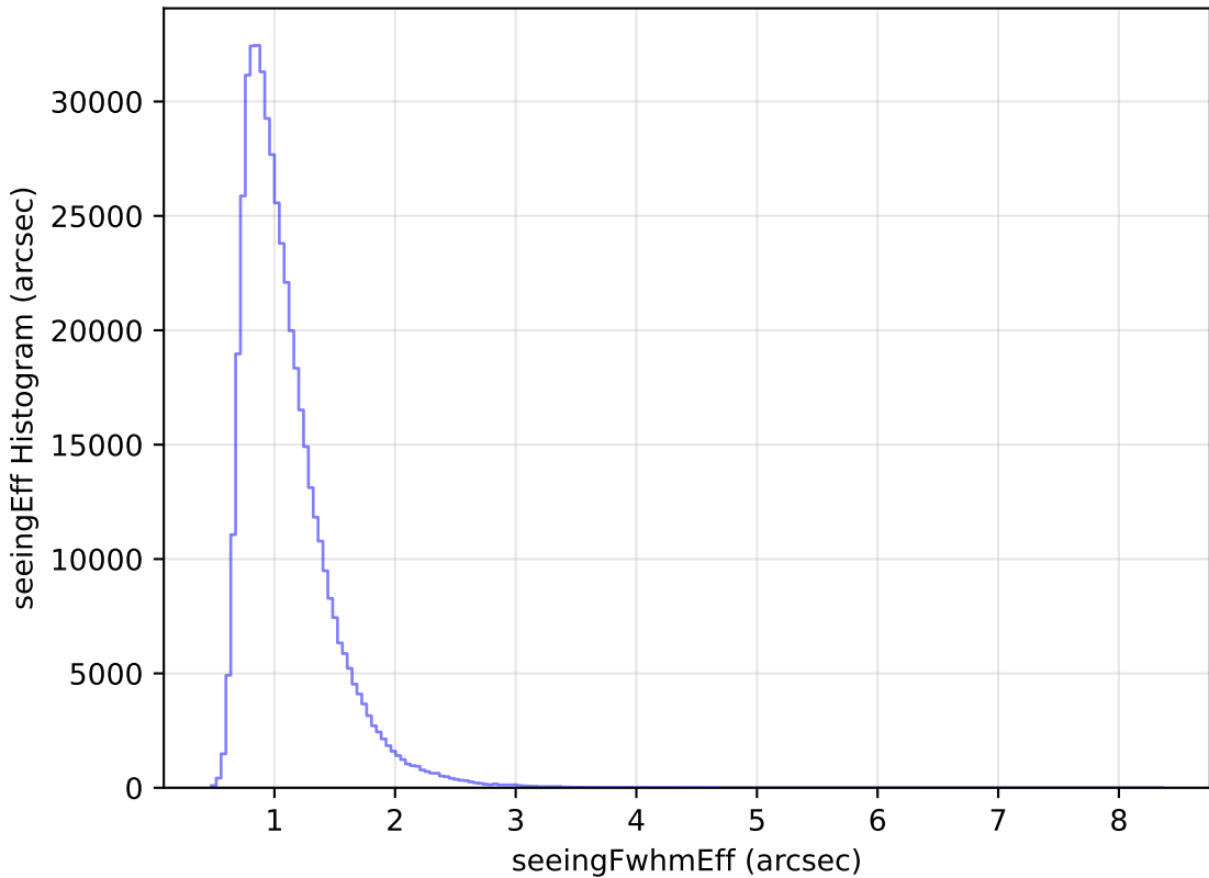
extra_ss_neo3_v3.4_10yrs WFD i band: seeingEff Histogram
