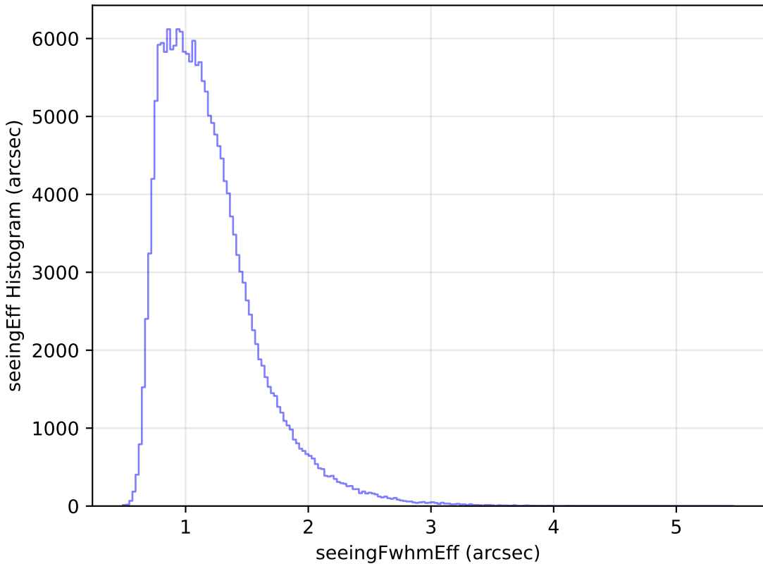
extra_ss_neo3_v3.4_10yrs WFD g band: seeingEff Histogram
