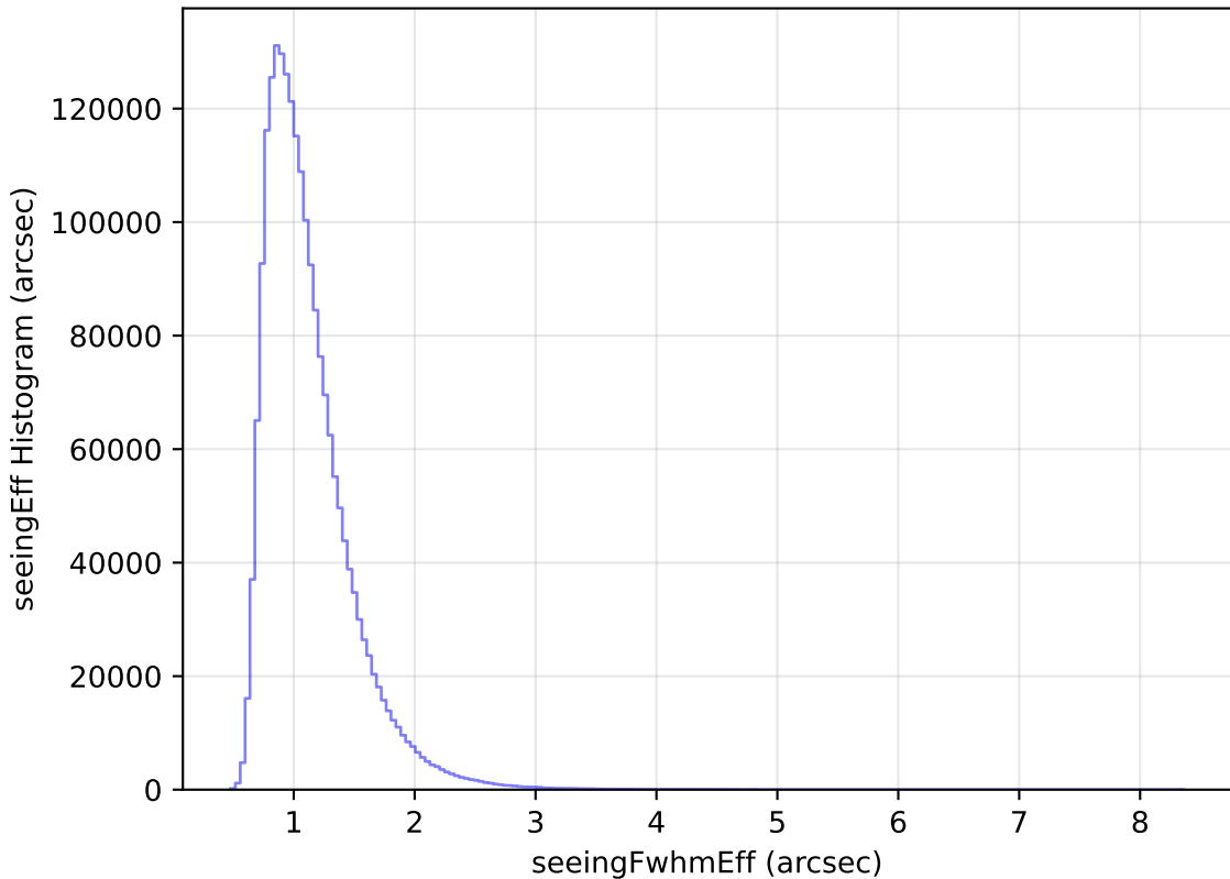
extra_ss_neo3_v3.4_10yrs WFD all bands: seeingEff Histogram
