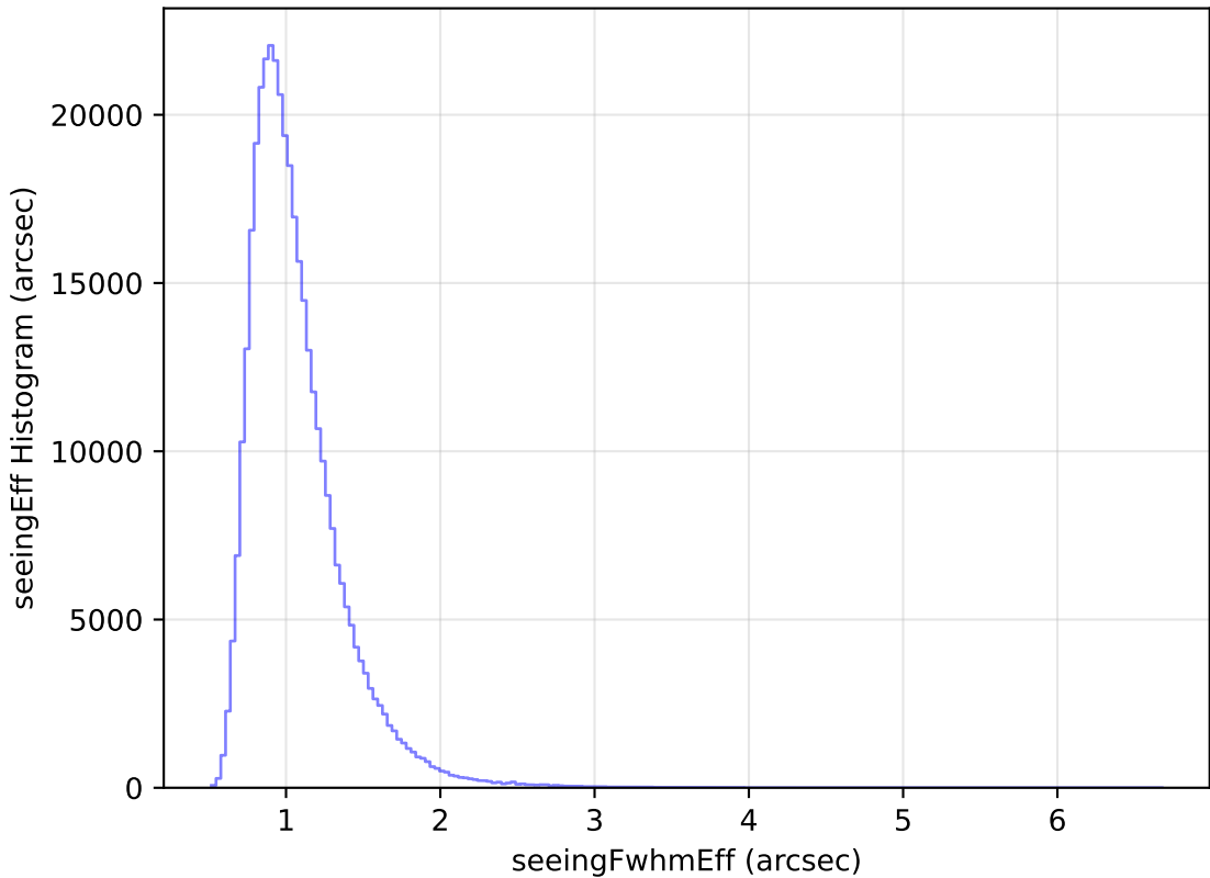
extra_ss_neo3_v3.4_10yrs All sky y band: seeingEff Histogram
