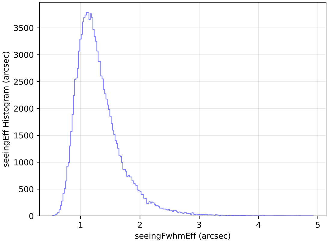
extra_ss_neo3_v3.4_10yrs All sky u band: seeingEff Histogram
