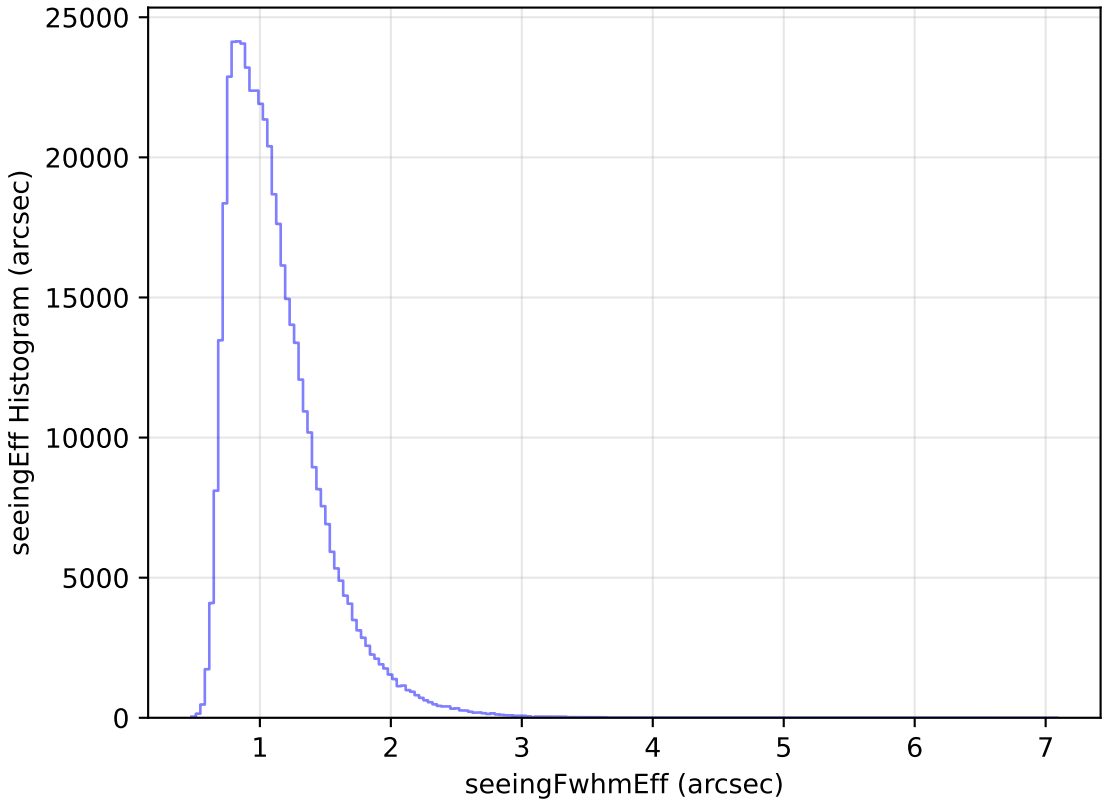
extra_ss_neo3_v3.4_10yrs All sky r band: seeingEff Histogram
