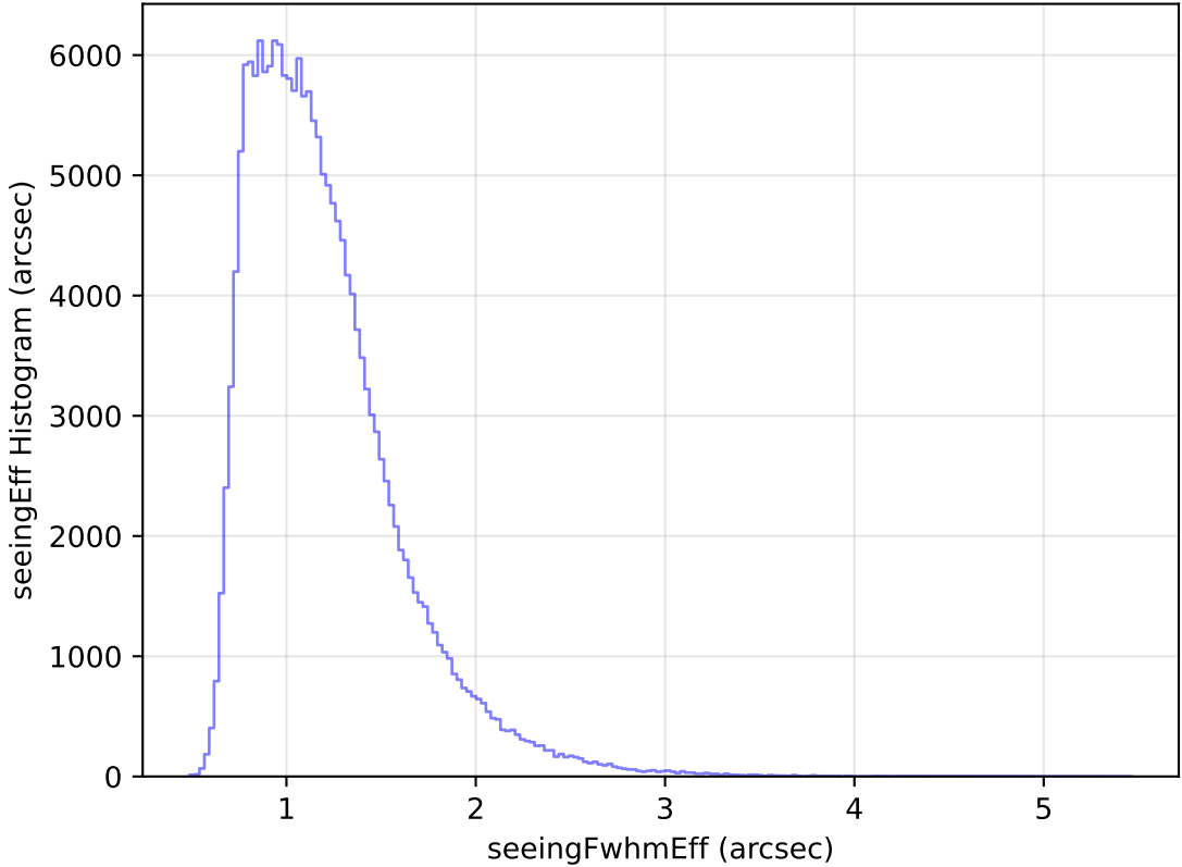
extra_ss_neo3_v3.4_10yrs All sky g band: seeingEff Histogram
