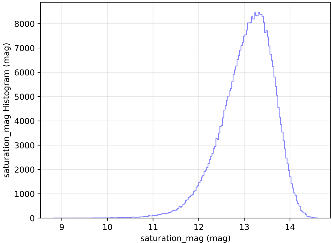
extra_ss_neo3_v3.4_10yrs WFD y band: saturation_mag Histogram
