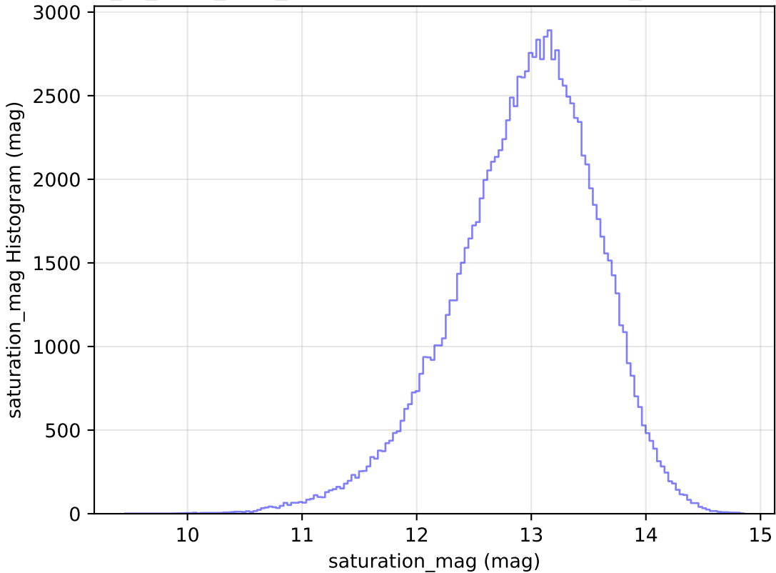
extra_ss_neo3_v3.4_10yrs WFD u band: saturation_mag Histogram
