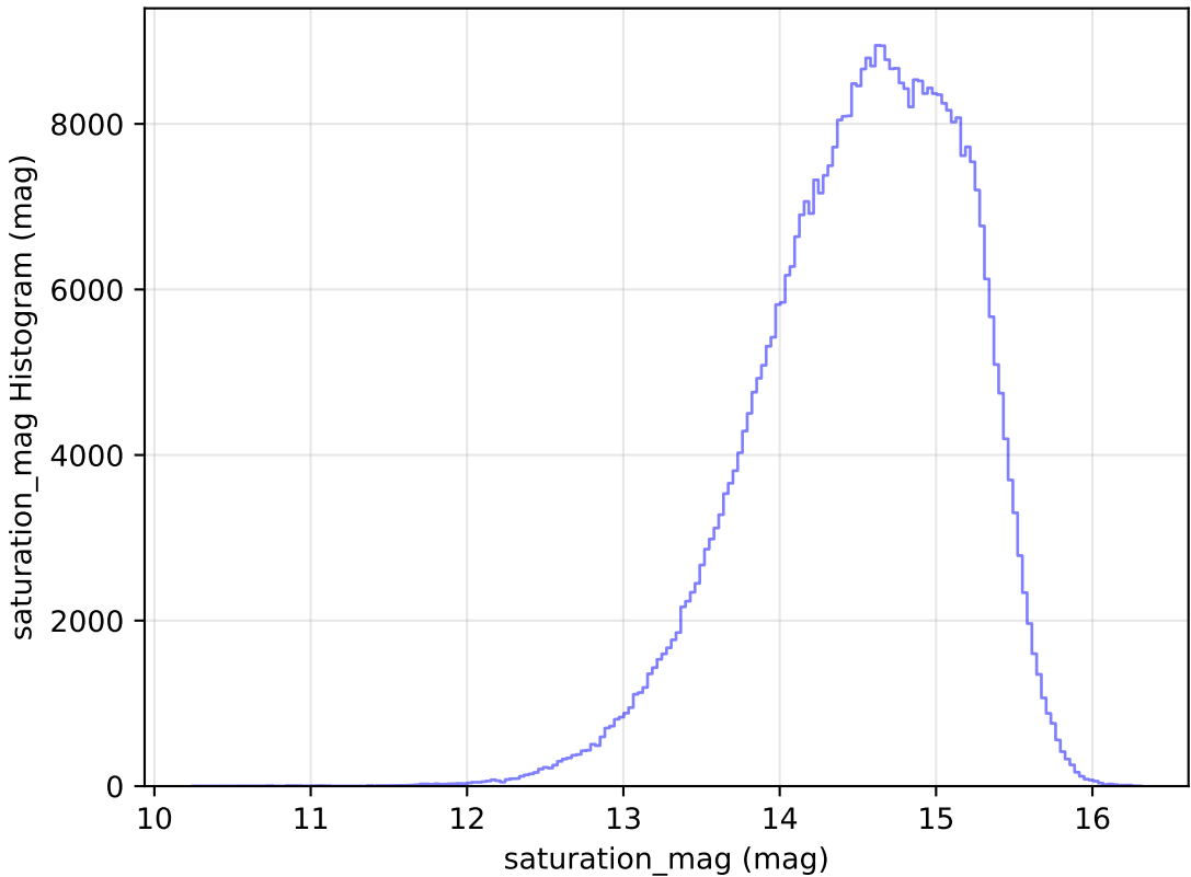
extra_ss_neo3_v3.4_10yrs WFD r band: saturation_mag Histogram
