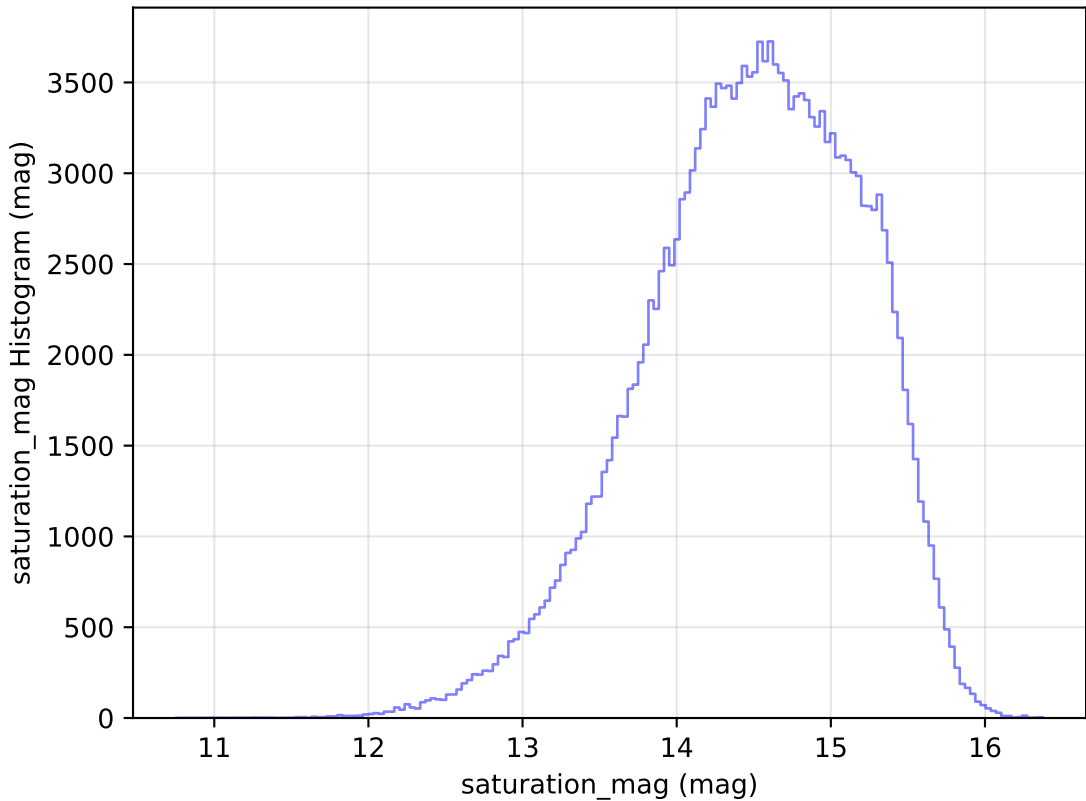
extra_ss_neo3_v3.4_10yrs WFD g band: saturation_mag Histogram
