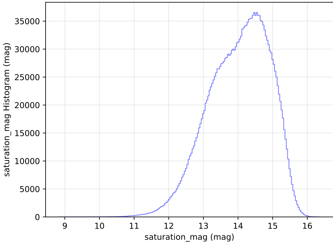
extra_ss_neo3_v3.4_10yrs WFD all bands: saturation_mag Histogram
