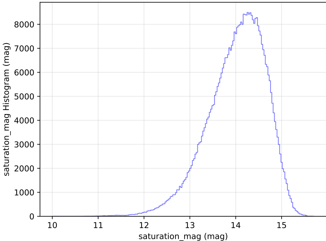
extra_ss_neo3_v3.4_10yrs All sky z band: saturation_mag Histogram
