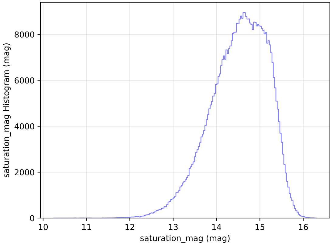
extra_ss_neo3_v3.4_10yrs All sky r band: saturation_mag Histogram
