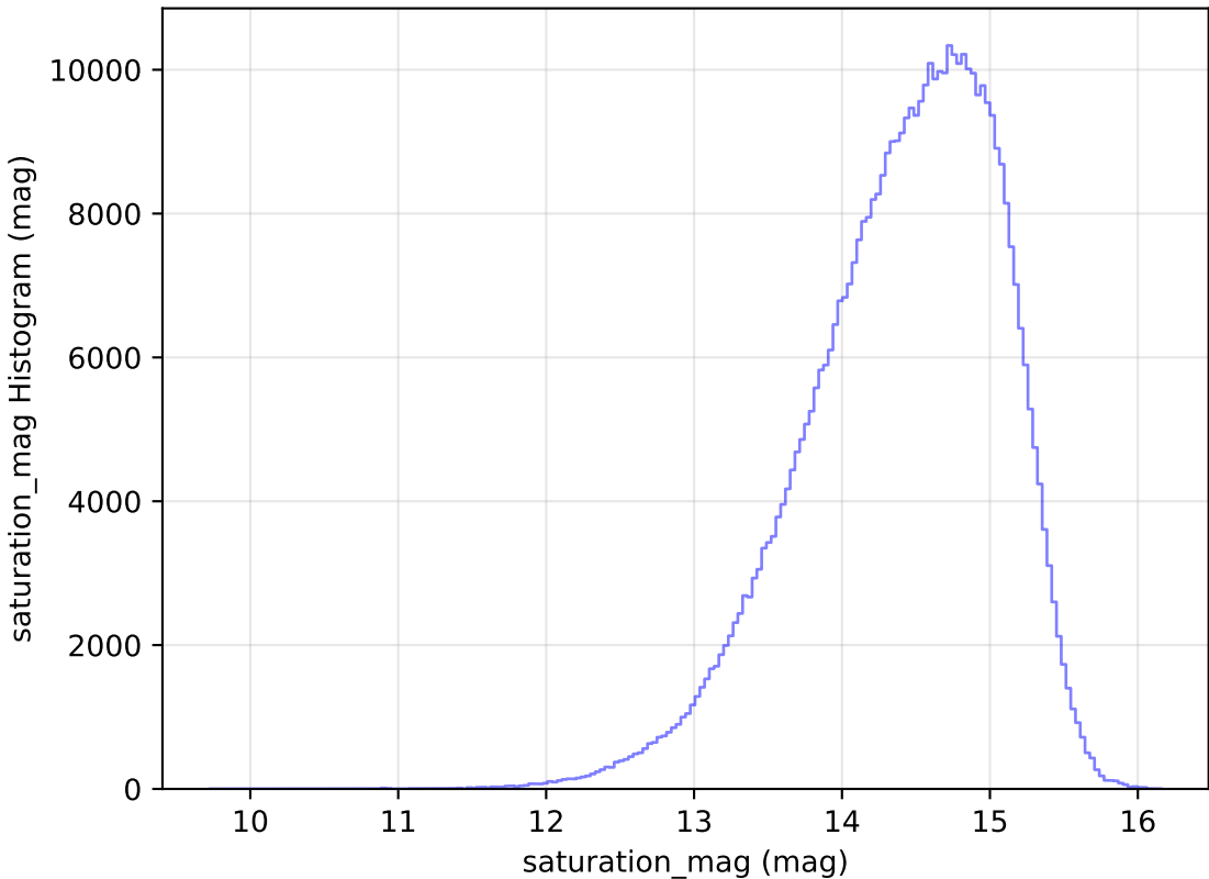
extra_ss_neo3_v3.4_10yrs All sky i band: saturation_mag Histogram
