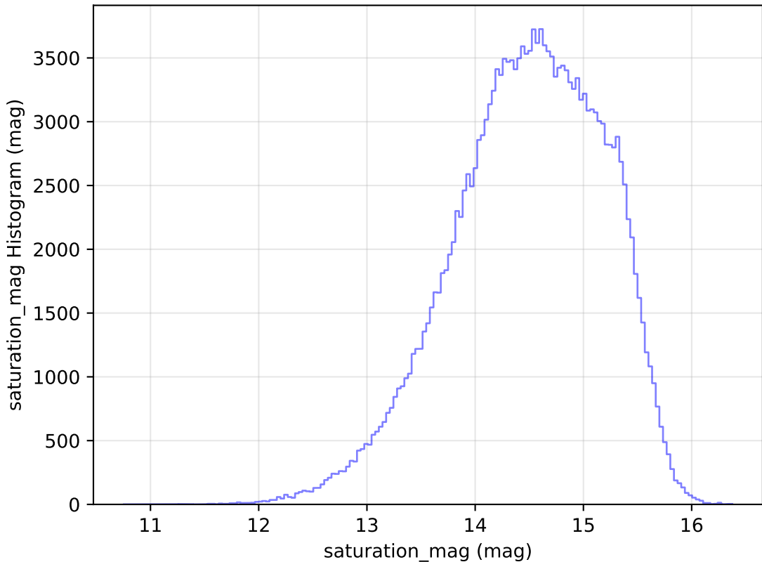
extra_ss_neo3_v3.4_10yrs All sky g band: saturation_mag Histogram
